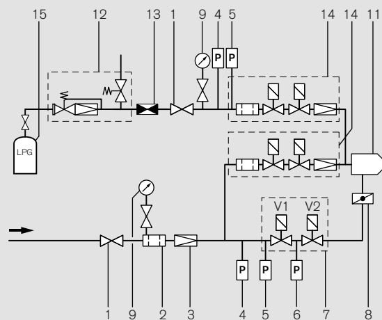
WKGMS 80, gas-side
