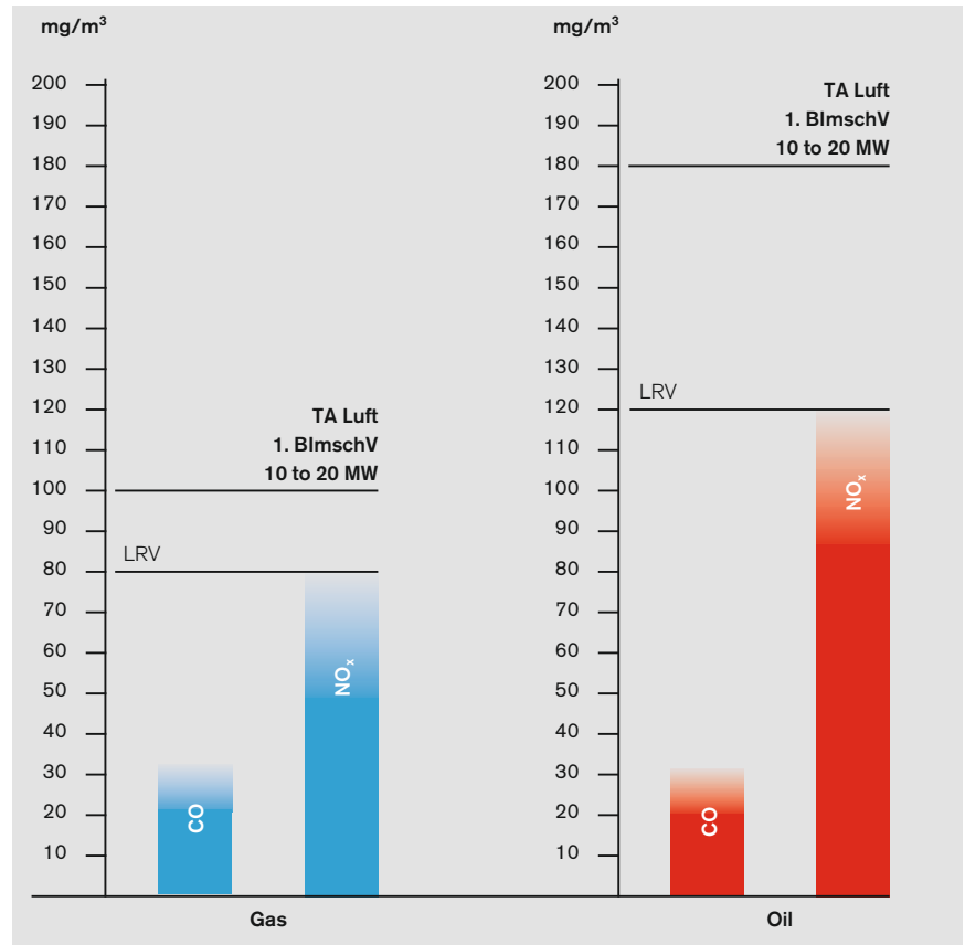
Typical emission levels for hot-water plant
