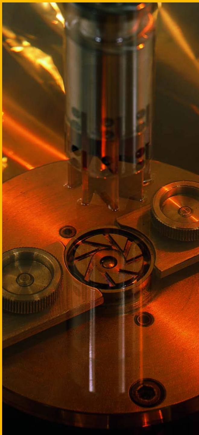
Manufacture of swirler plates for Weishaupt industrial burner nozzles: here the highest precision is required.
